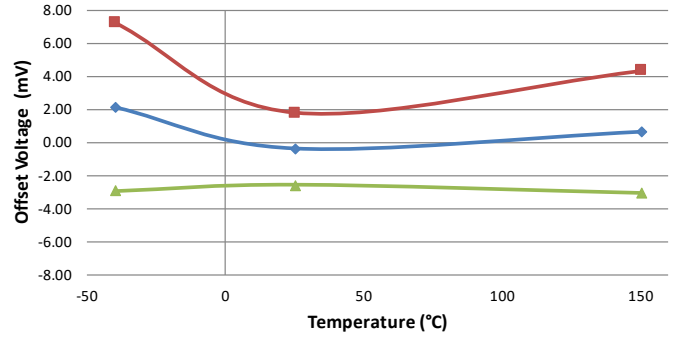
Offset Voltage vs. Temperature
